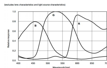
MV-SUA2000C
