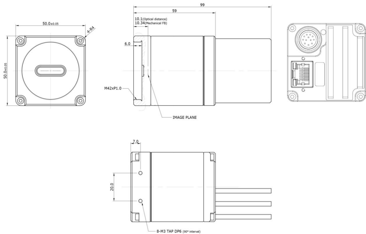
Figure 5-4 Mechanical Dimension
