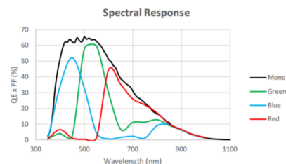
MV-XGC6500GC/GM
