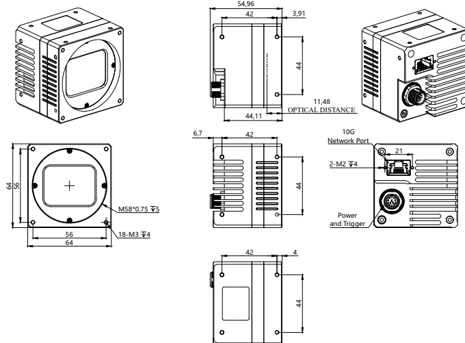
MV-XGC6500GC/GM-T-M58
