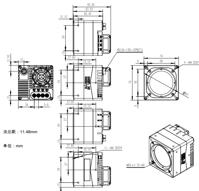
MARS-6503-71X2M/C-NF (M58 口带风扇)
