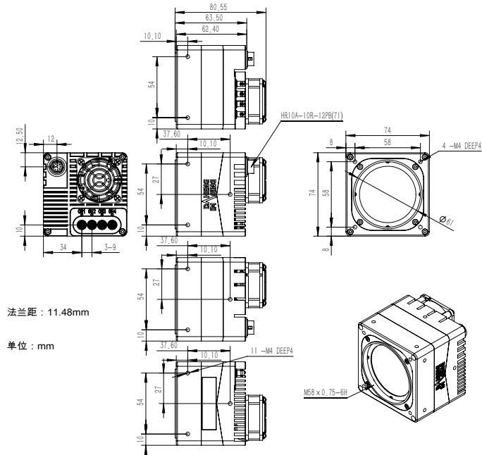
MARS-6502-71X2M/C-NF (M58 口带风扇)
