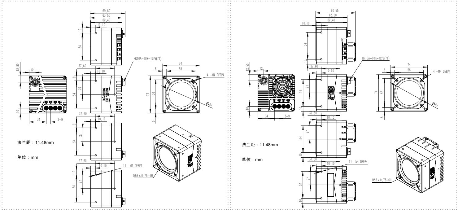
MARS-6502-71X2M/C (M58 口)
