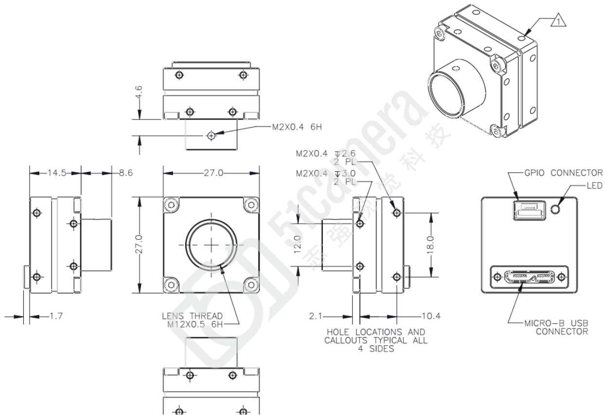
Firefly Dimensional Drawing S-mount
