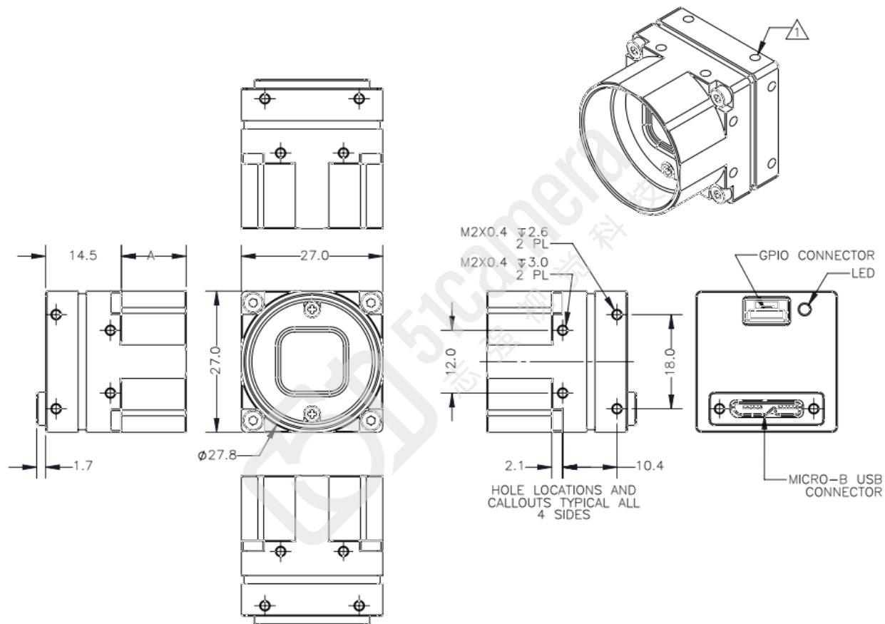
Firefly Dimensional Drawing C-mount
