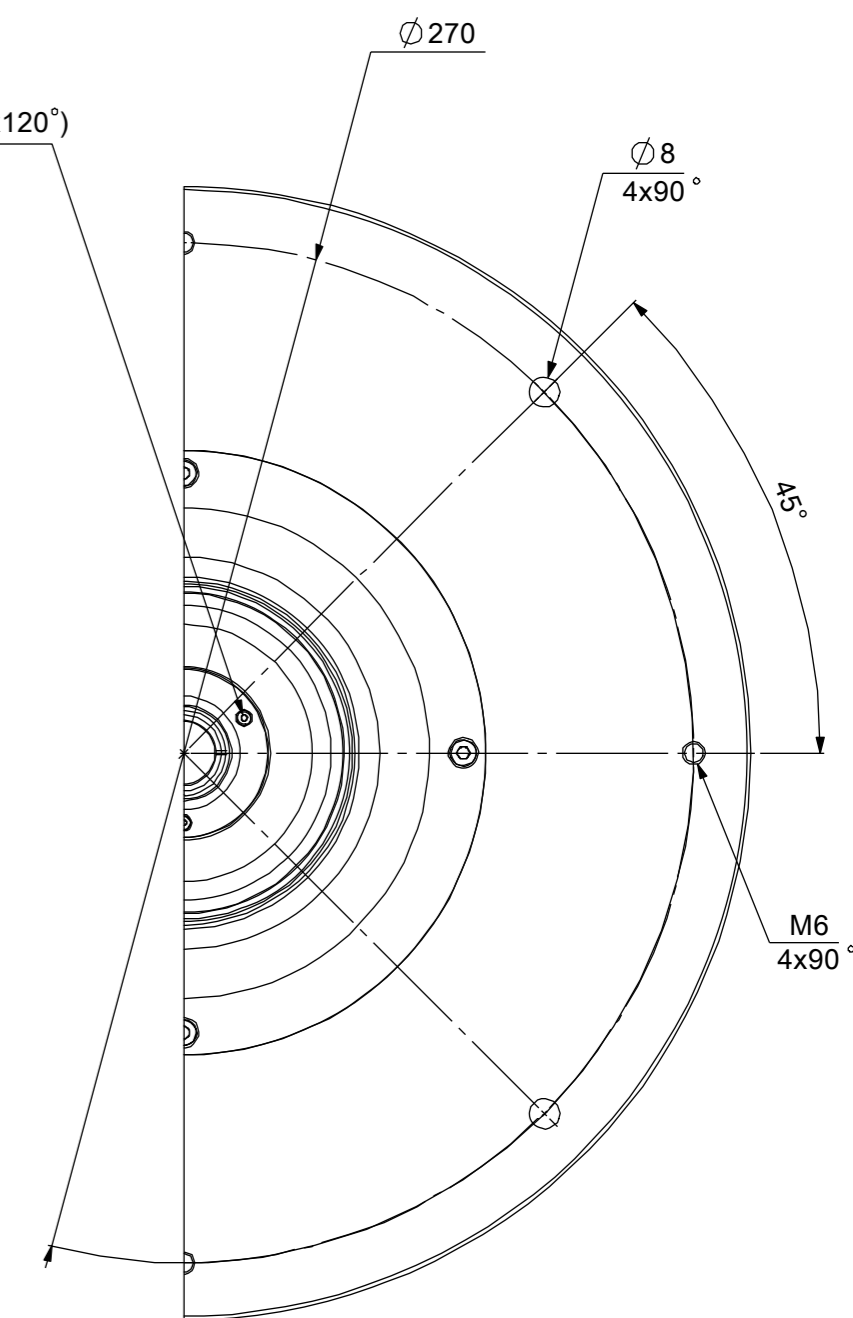
MOUNTING PORTION DETAIL VIEW フランジ取付部詳細
