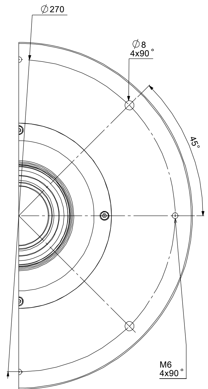
MOUNTING PORTION DETAIL VIEW
