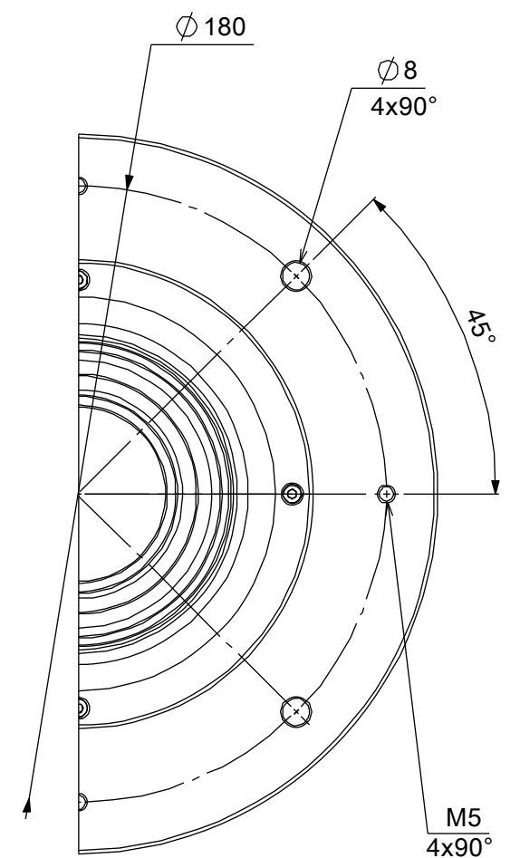
MOUNTING PORTION DETAIL VIEW フランジ取付部詳細
