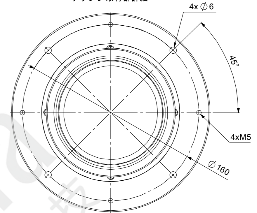
VIEW A
