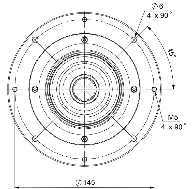
MOUNTING PORTION DETAIL VIEW フランジ取付部詳細
