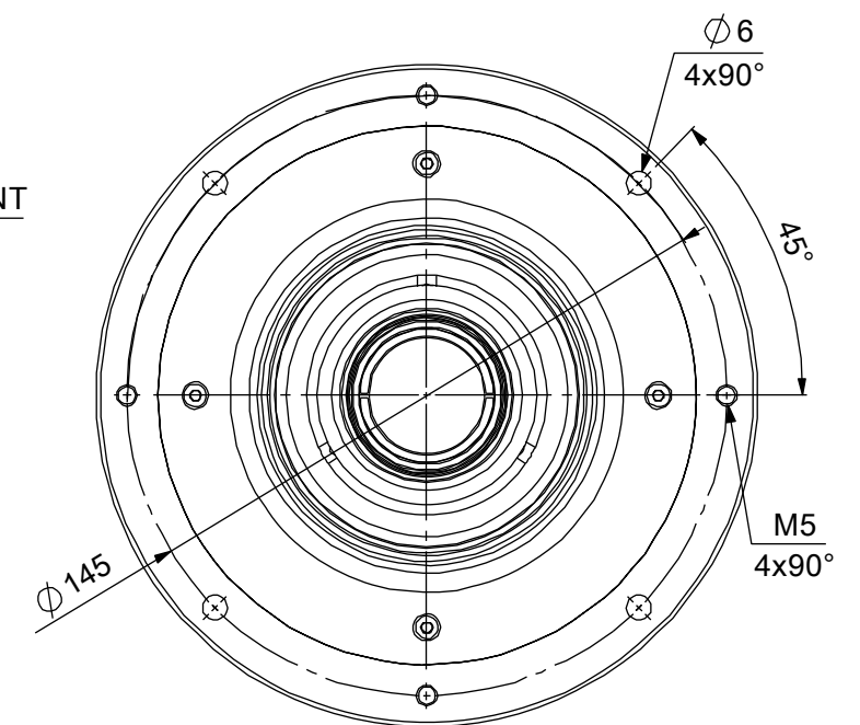
MOUNTING PORTION DETAIL VIEW
