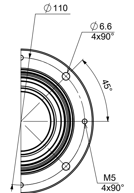
MOUNTING PORTION DETAIL VIEW フランジ取付部詳細
