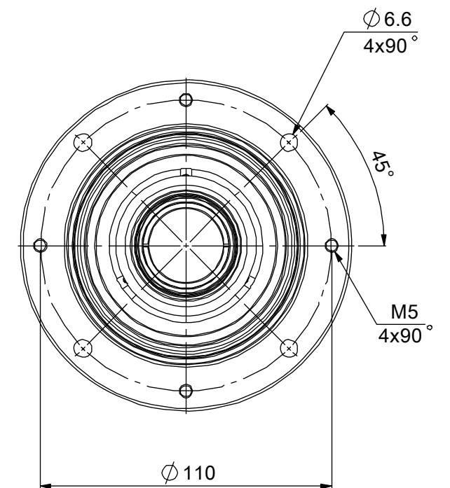
MOUNTING PORTION DETAIL VIEW
