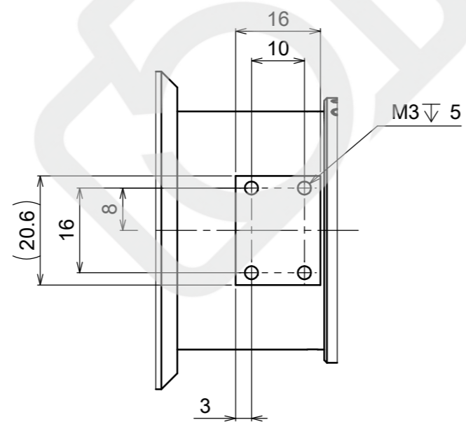
VIEW A (1:1)
