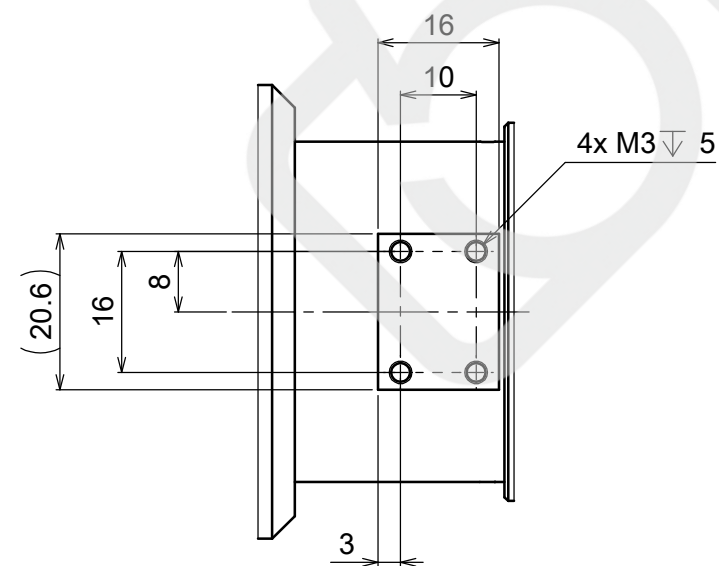
VIEW A
