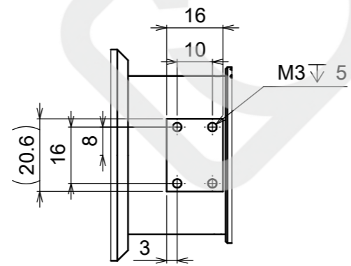
VIEW A
