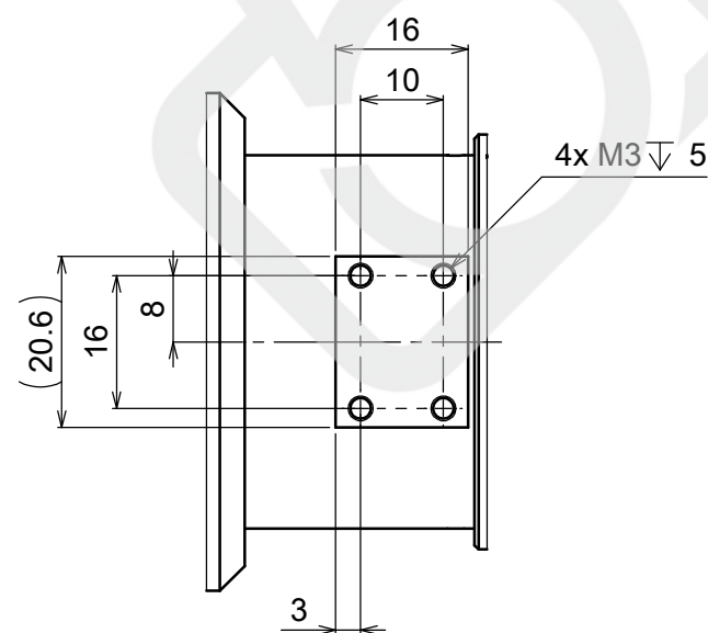
VIEW A
