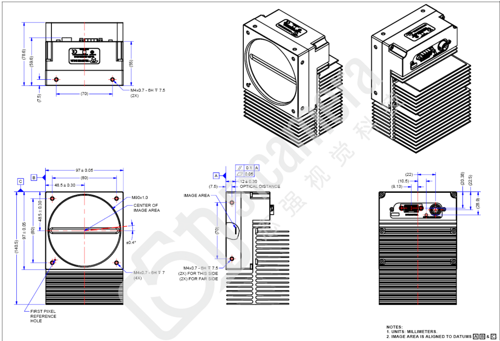
HL-HM-13K30H-00-R, HL-HM-16K30H-00-R, HL-HM-16K40H-00-R and HL-HF-16K10T-00-R Mechanical Drawing
