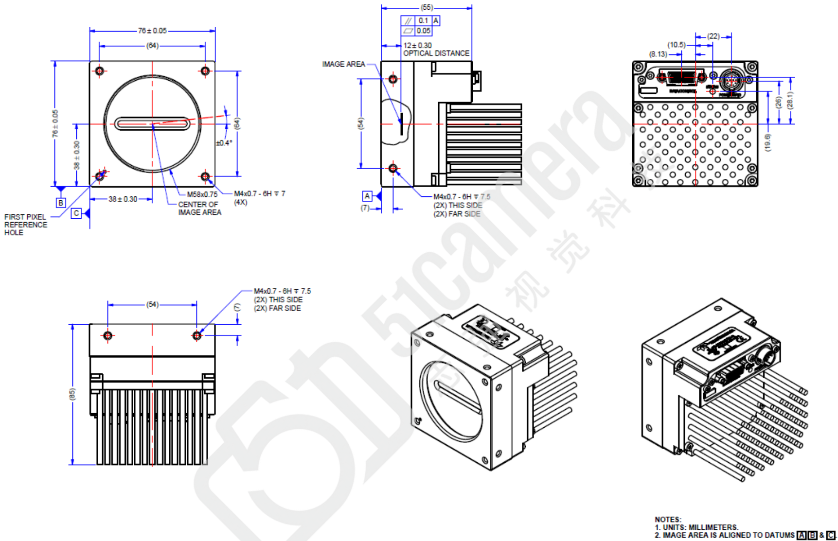
HL-HM-08K30H-00-R and HL-HM-08K40H-00-R Mechanical Drawing
