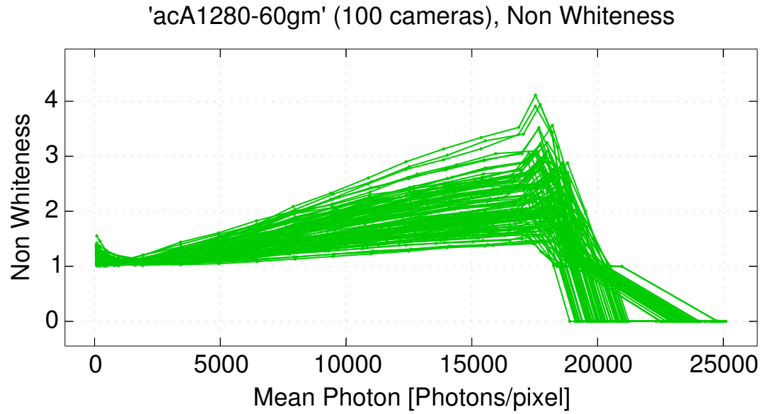
Figure 11: Non-whiteness Coefficient
