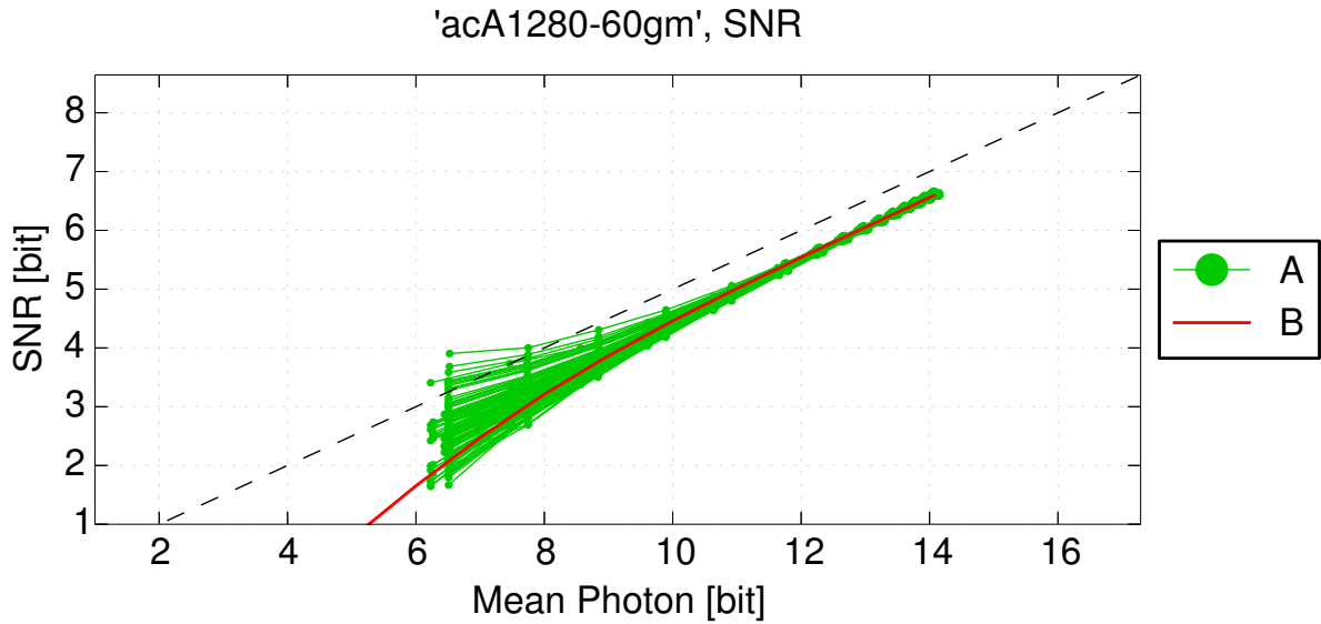
Figure 13: Signal-to-noise Ratio
