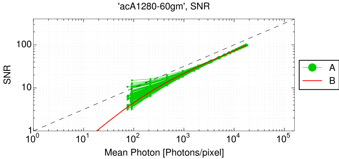
Figure 14: Signal-to-noise Ratio
