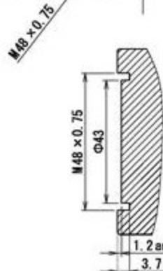
Lens mount cross-section diagram
