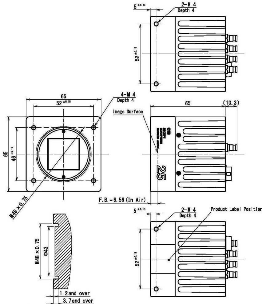
Lens mount cross-section diagram
