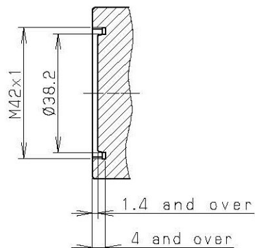
Lens mount cross-section diagram
