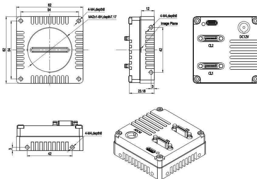
PL4KCL Camera Mechanical Dimensions (in mm)
