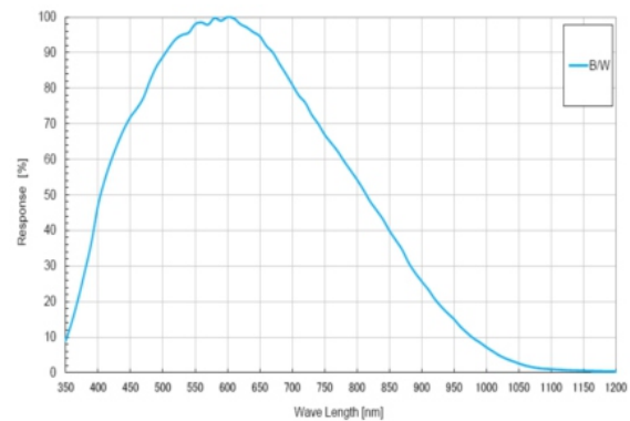
MV-GED32M-T
