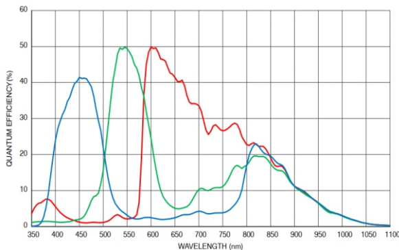
Figure 50. Quantum Efficiency (Color)
