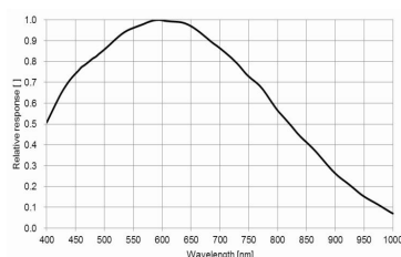
MER2-502-79U3M-L
