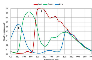
MER2-502-79U3C-L
