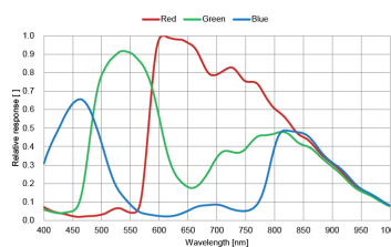
MER2-160-227U3C
